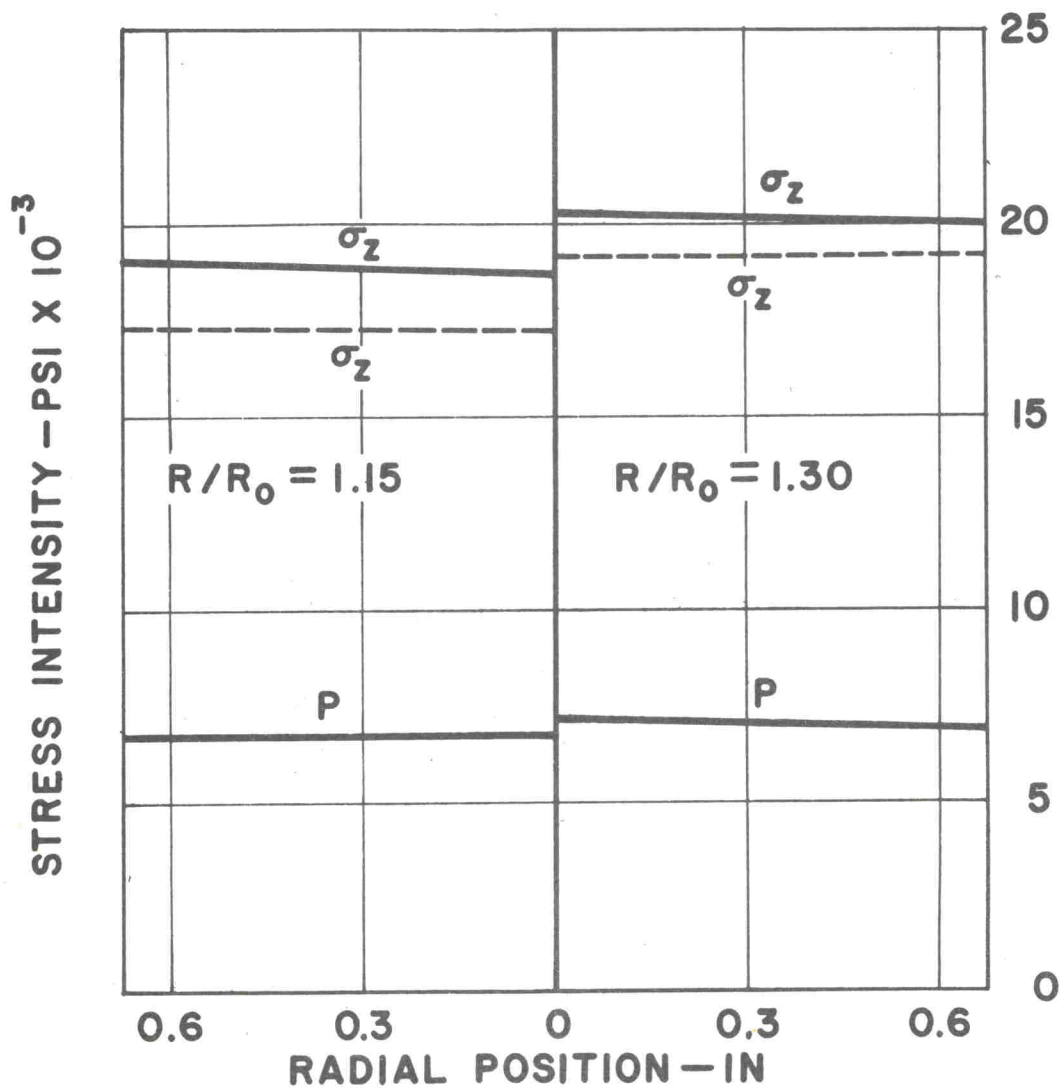
FIG. 20 ONE-DIMENSIONAL STRESS DISTRIBUTION FOR 2S ALUMINUM. CASE I-A.
